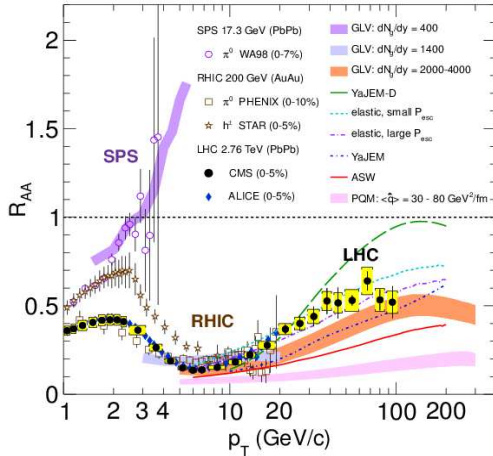
Fig 1. CMS: The nuclear modification factor R_{AA} in central heavy-ion collisions for neutral and charged hadrons, at several center-of-mass energies.
