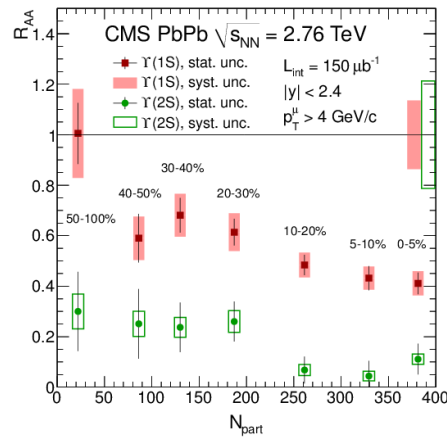
Fig 2. CMS: The nuclear modification factor R_{AA} for upsilon states as a function of the centrality of the heavy-ion collision.
